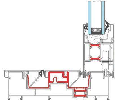
B45 TRI-RAIL
