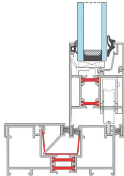
B45 DUO-RAIL
