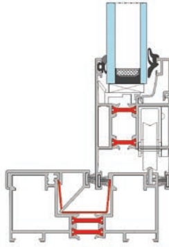
B45 DUO-SCHIENE
