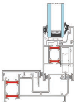
B45 MONO-SCHIENE
